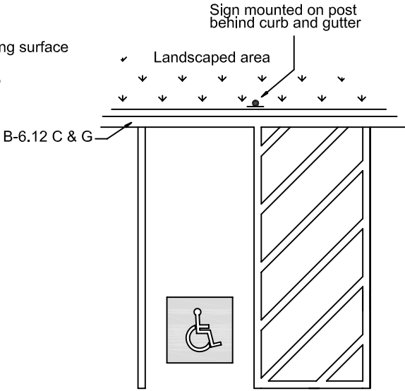
Behind curb & gutter
